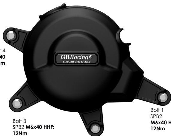
Bolt 2 SPB2 M6x40 HHF: 12Nm
